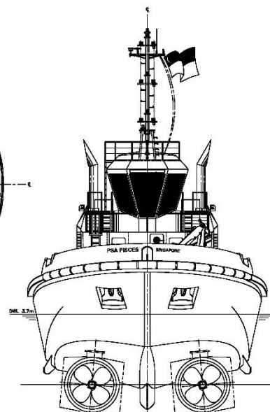
STERN VIEW
