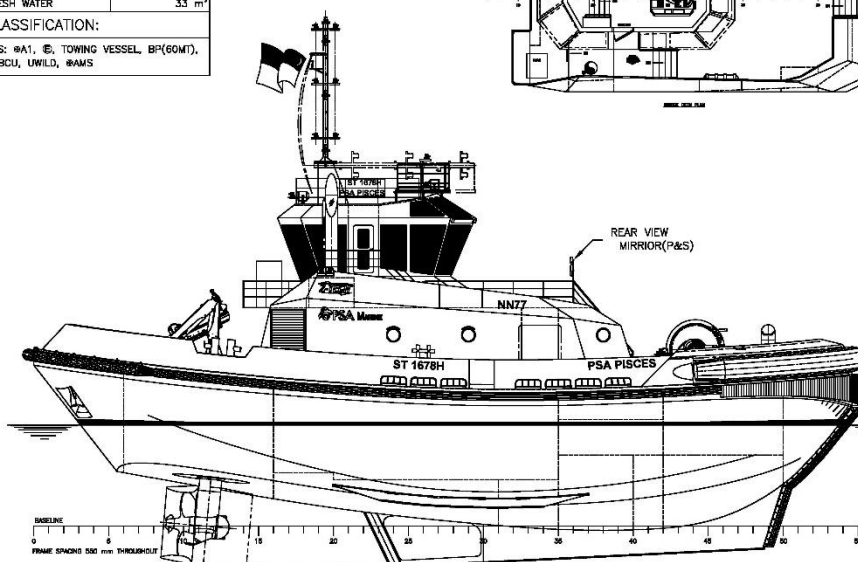
OUTBOARD PROFILE
