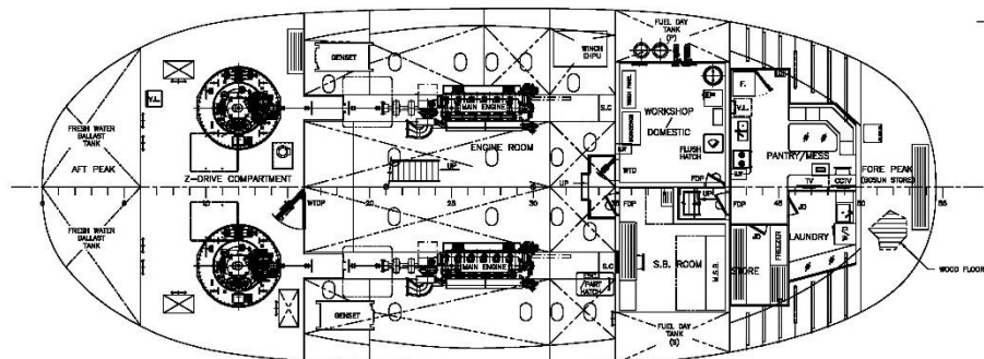
HOLD PLAN
