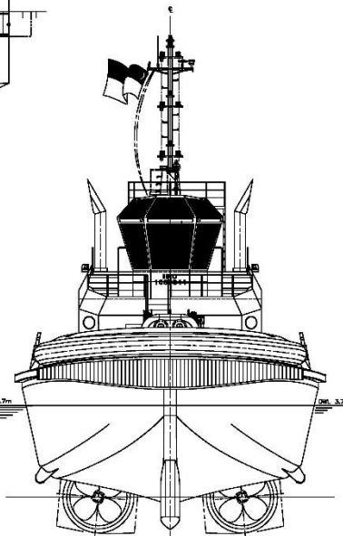
BOW VIEW
