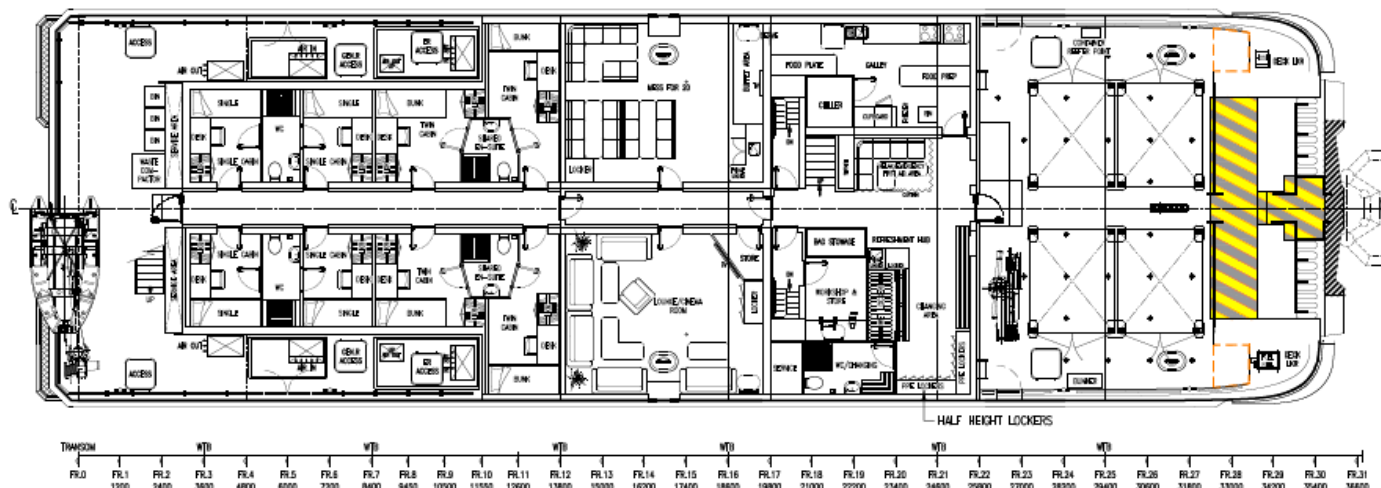
PLAN VIEW ON MAIN DECK
