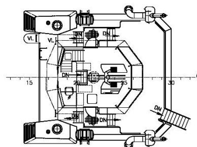
BRIDGE DECK
