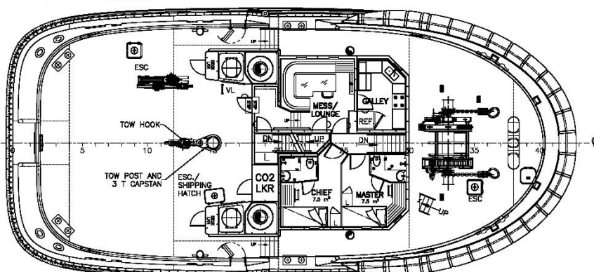
MAIN DECK PLAN
