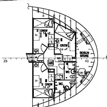
LOWER ACCOMMODATIONS
