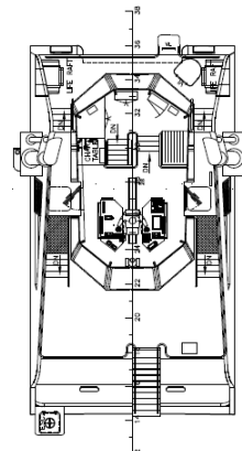
WHEELHOUSE PLAN
