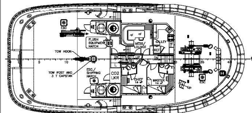
MAIN DECK PLAN
